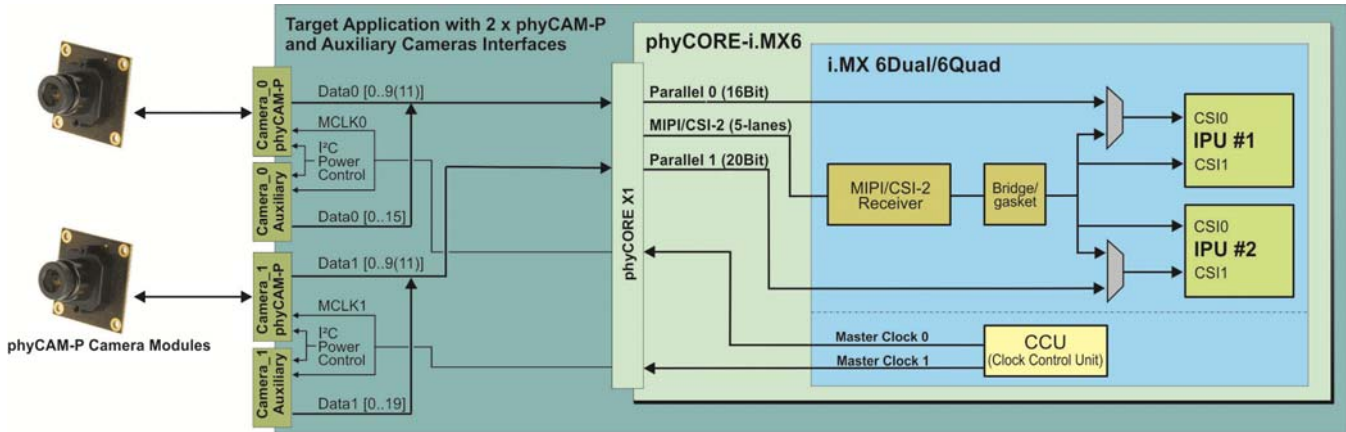
Figure 13: Use of Parallel 0 (CSIO of IPU#1) and Parallel 1 (CSI1 of IPU#2) as phyCAM-P interface
