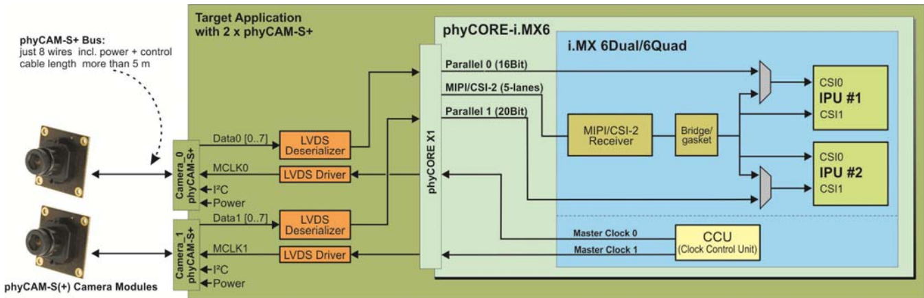
Figure 14: Use of Parallel 0 (CSIO of IPU#1) and Parallel 1 (CSI1 of IPU#2) as phyCAM-S+ interface
